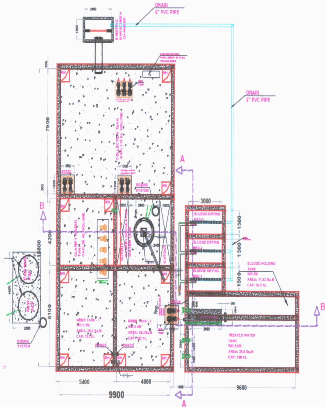
WASTE WATER RECYCLING PLANT LAYOUT
